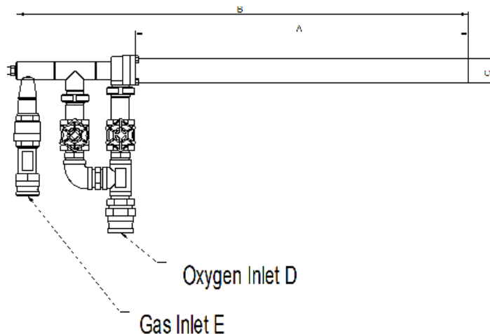
Figure 1: FFO57 Series Oxygen-Gas Burner
