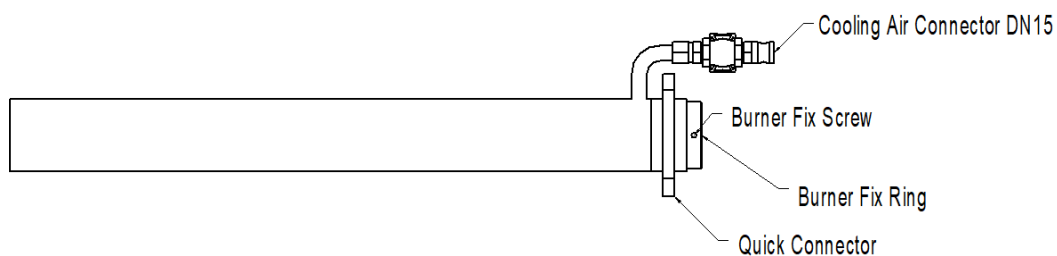
Figure 2: FFO57 Series Oxygen-Natural Gas Burner mounting sleeve
